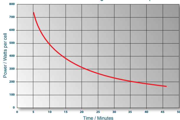
NSB12-330FT Discharge Curve to 1.67 vpc
